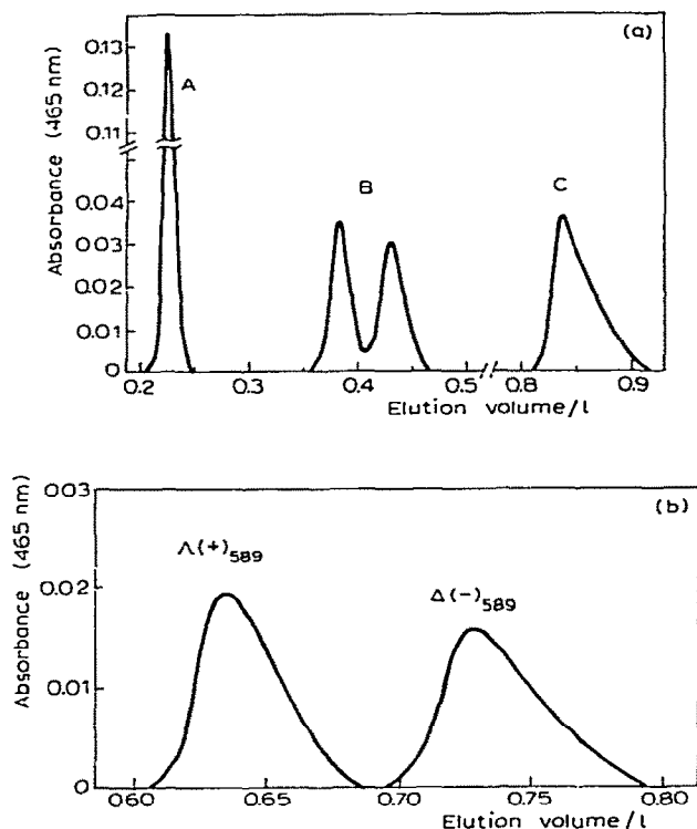
Fig. 2. Elution curves of [\text{Co}(\text{en})_3]^{3+} on an SE-Sephadex column. (a) Eluent: A, 0.2 M sodium sulfate; B, 0.2 M sodium (+)-tartrate; C, 0.4 M sodium chloride. (b) Eluent: 0.15 M sodium (+)-tartrate.
